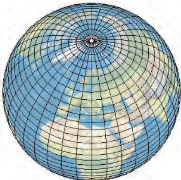
Figure 1.10 : The Graticule
