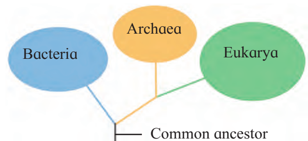
Fig 2.1 Phylogenetic descent
